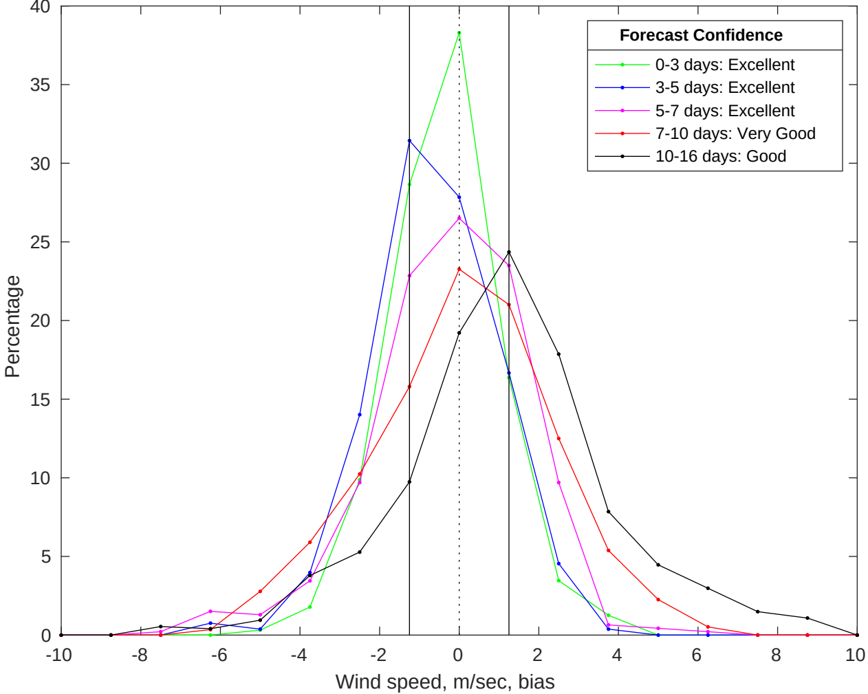
NDBC 42035 vs GFS Winds Bias Histogram: 04-Jul-2025
