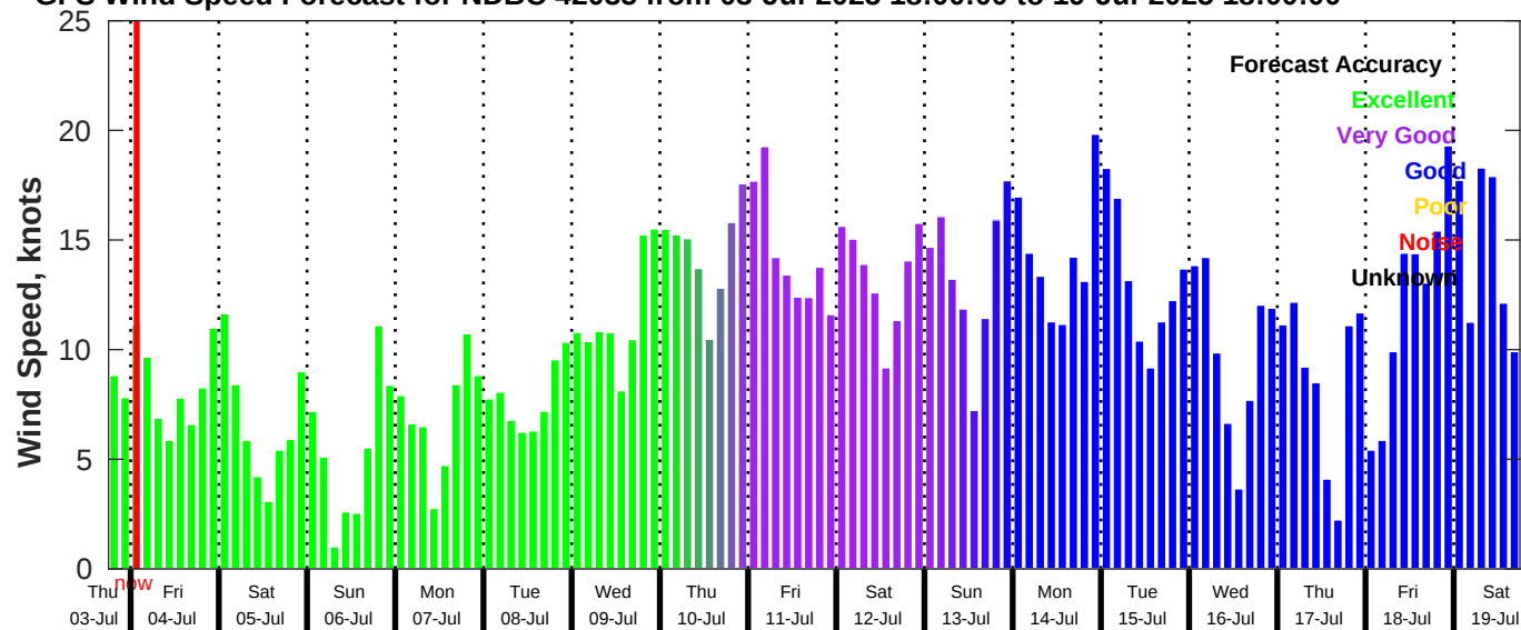
GFS Wind Speed Forecast for NDBC 42035 from 03-Jul-2025 18:00:00 to 19-Jul-2025 18:00:00
