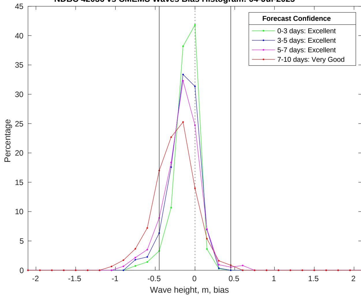
NDBC 42036 vs CMEMS Waves Bias Histogram: 04-Jul-2025
