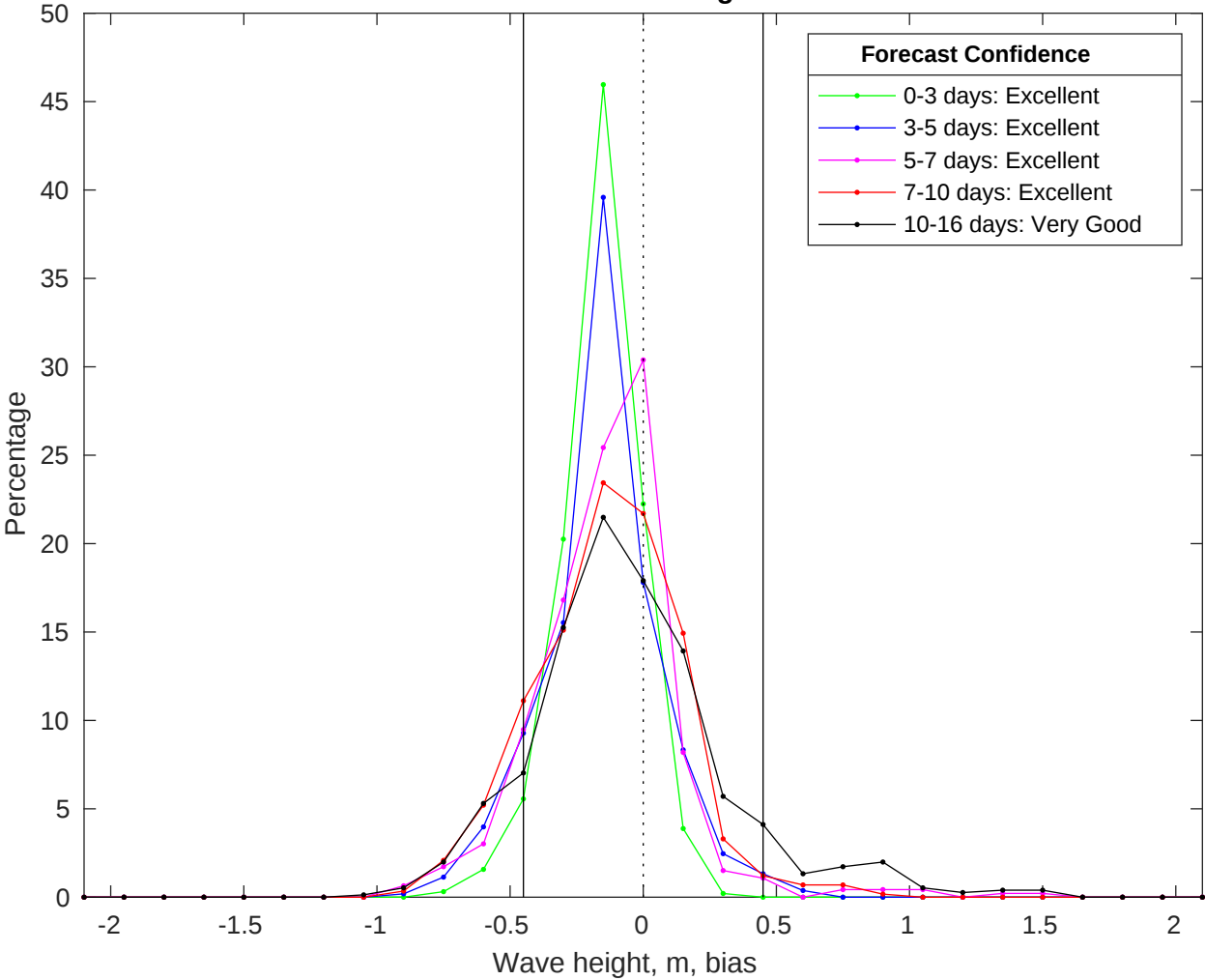
NDBC 42036 vs GFS Waves Bias Histogram: 04-Jul-2025
