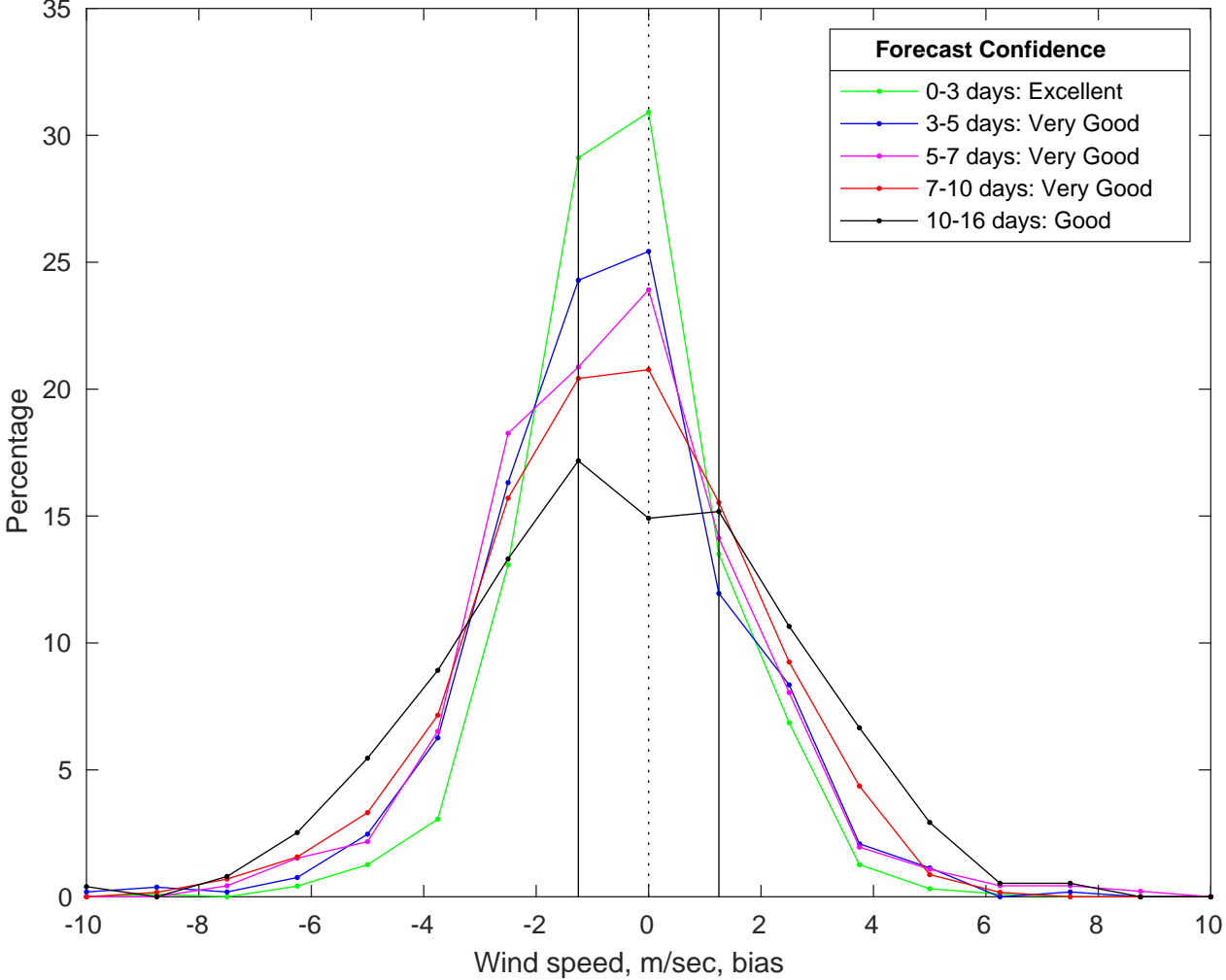
NDBC 42036 vs GFS Winds Bias Histogram: 04-Jul-2025
