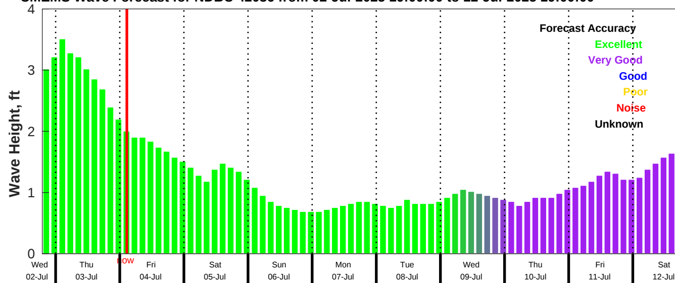
CMEMS Wave Forecast for NDBC 42036 from 02-Jul-2025 19:00:00 to 12-Jul-2025 19:00:00
