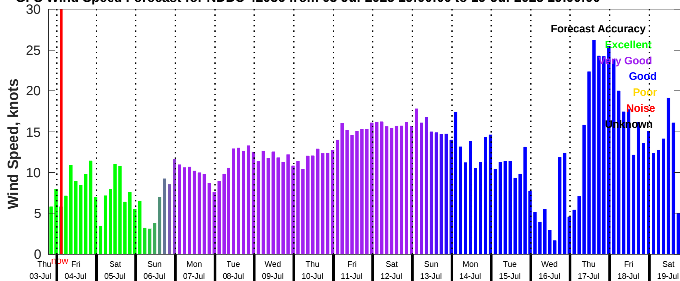
GFS Wind Speed Forecast for NDBC 42036 from 03-Jul-2025 19:00:00 to 19-Jul-2025 19:00:00
