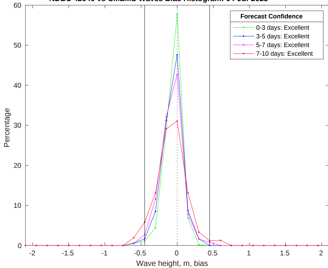
NDBC 42040 vs CMEMS Waves Bias Histogram: 04-Jul-2025
