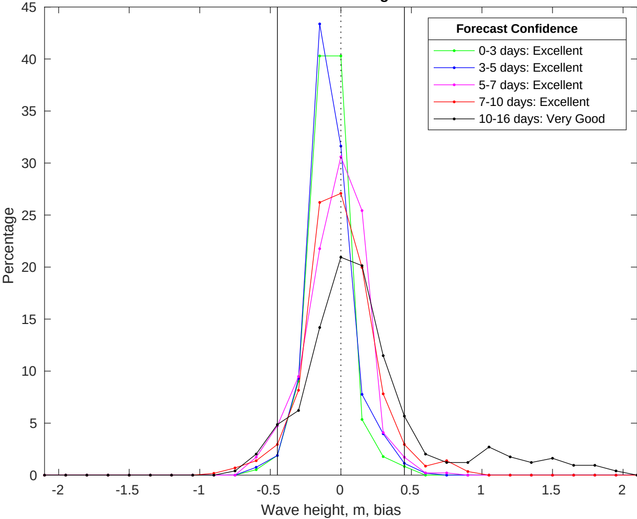
NDBC 42040 vs GFS Waves Bias Histogram: 04-Jul-2025
