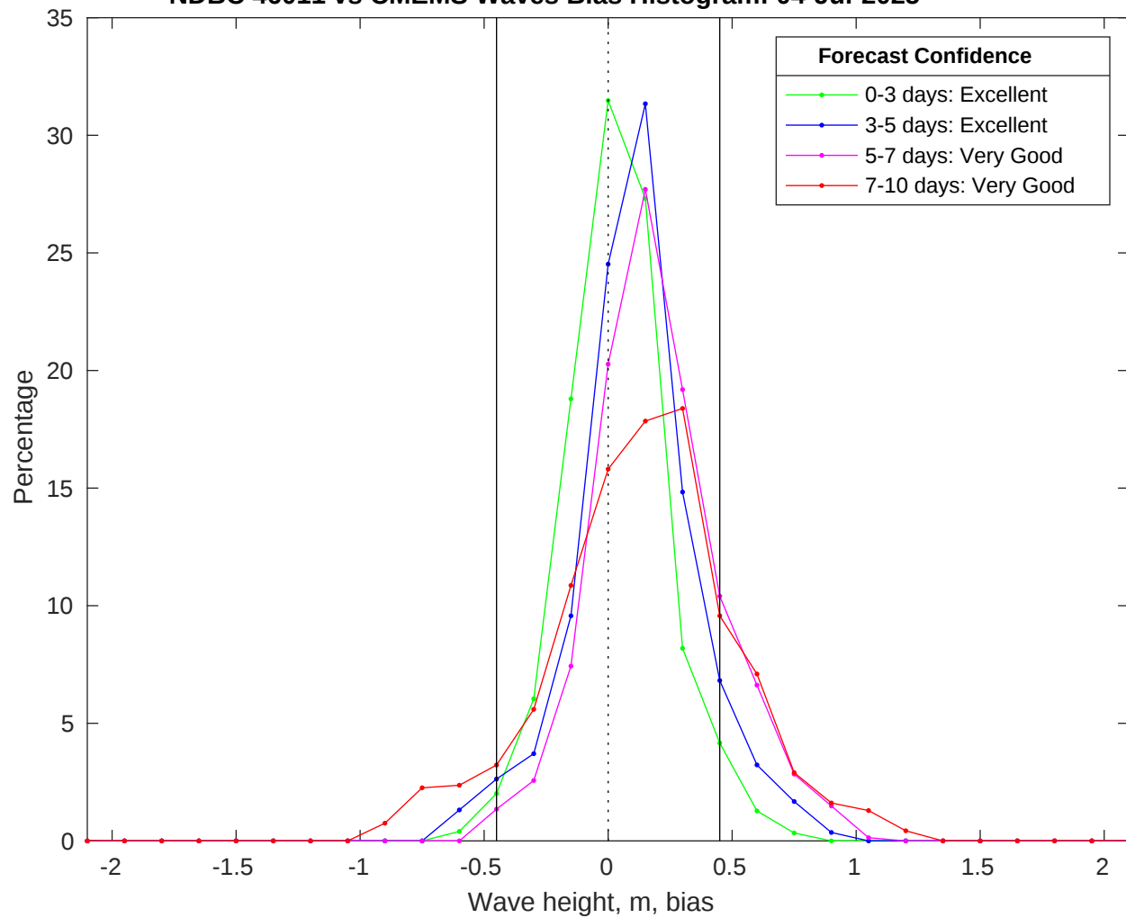
NDBC 46011 vs CMEMS Waves Bias Histogram: 04-Jul-2025
