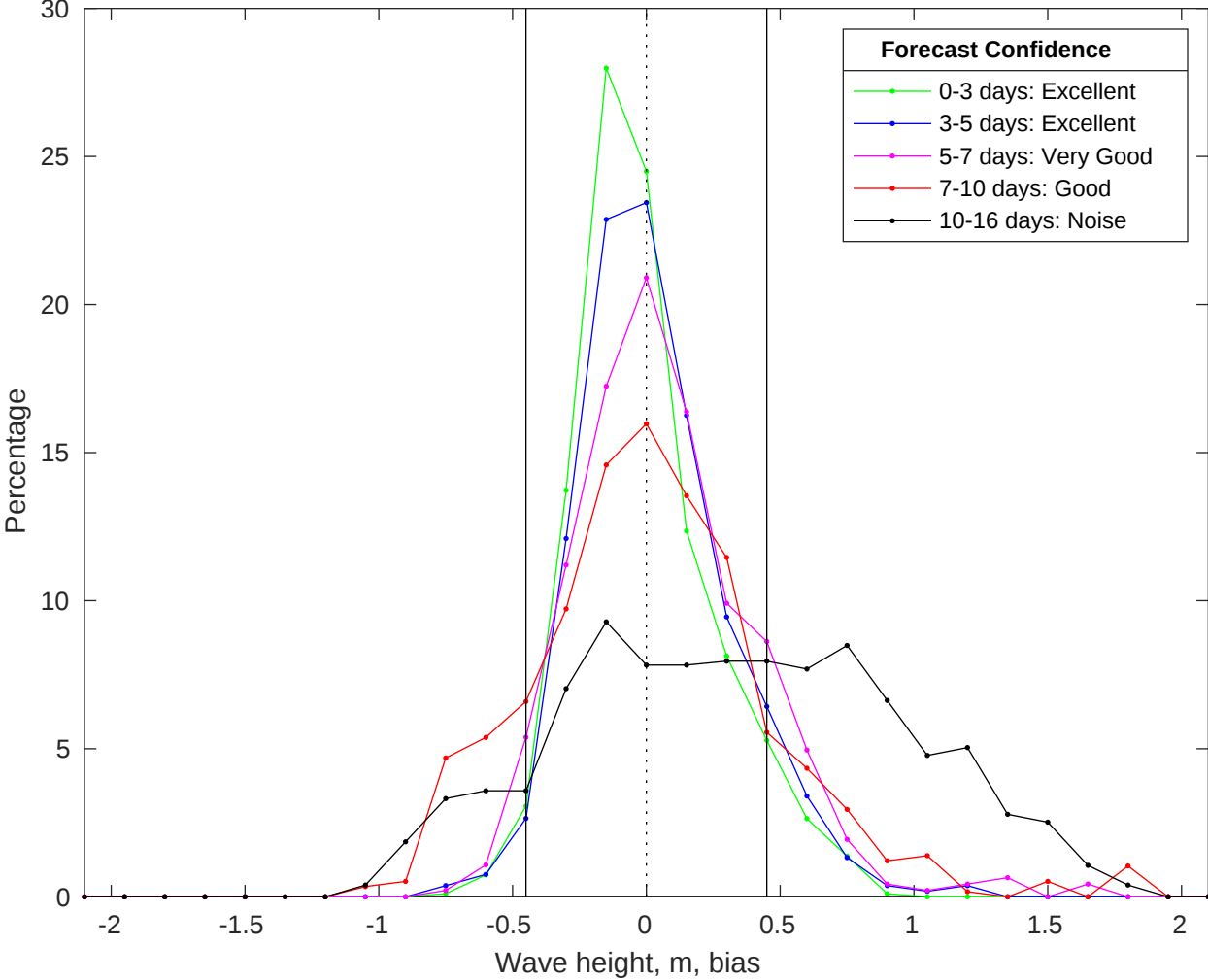
NDBC 46011 vs GFS Waves Bias Histogram: 04-Jul-2025
