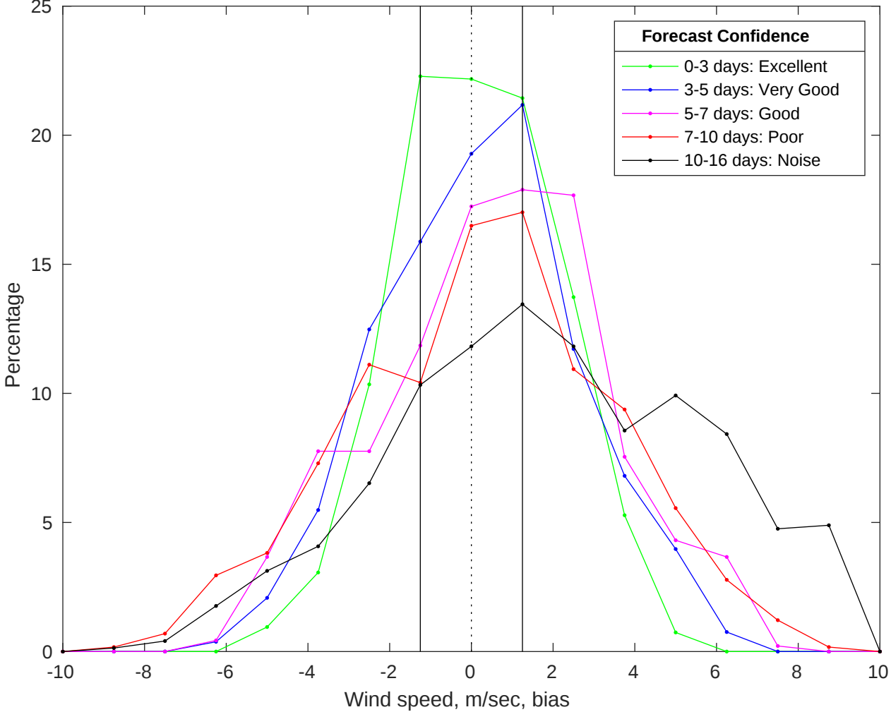
NDBC 46011 vs GFS Winds Bias Histogram: 04-Jul-2025
