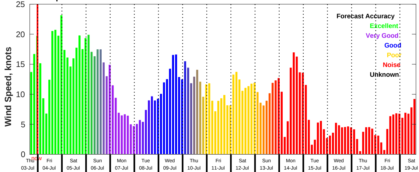
GFS Wind Speed Forecast for NDBC 46011 from 03-Jul-2025 16:00:00 to 19-Jul-2025 16:00:00
