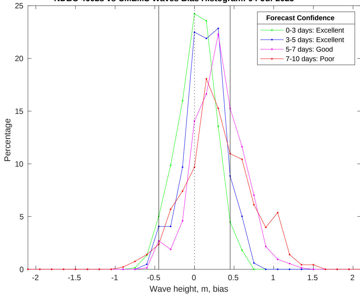
NDBC 46028 vs CMEMS Waves Bias Histogram: 04-Jul-2025
