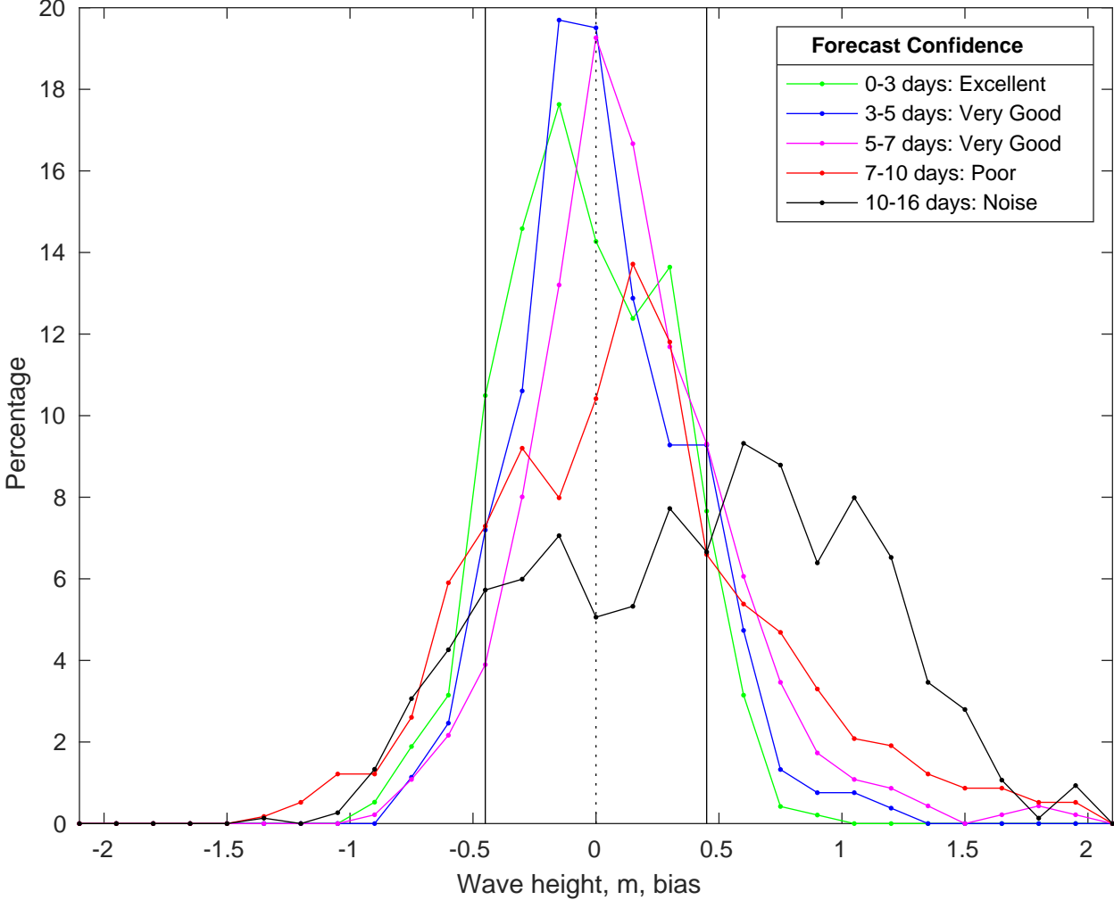
NDBC 46028 vs GFS Waves Bias Histogram: 04-Jul-2025
