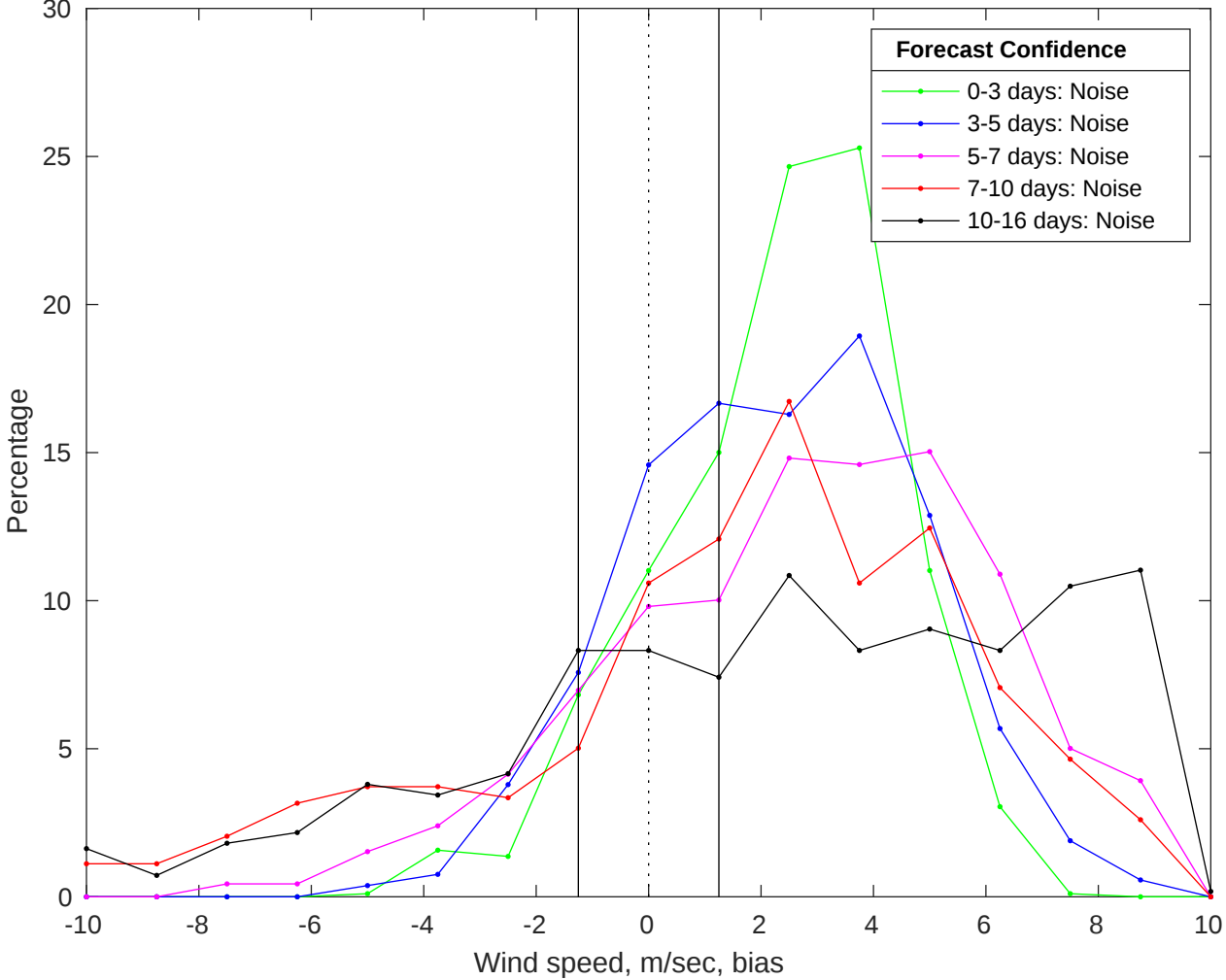
NDBC 46028 vs GFS Winds Bias Histogram: 04-Jul-2025
