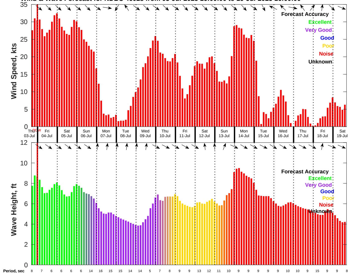
Wind & Wave Forecast for NDBC 46028 from 03-Jul-2025 16:00:00 to 19-Jul-2025 16:00:00
