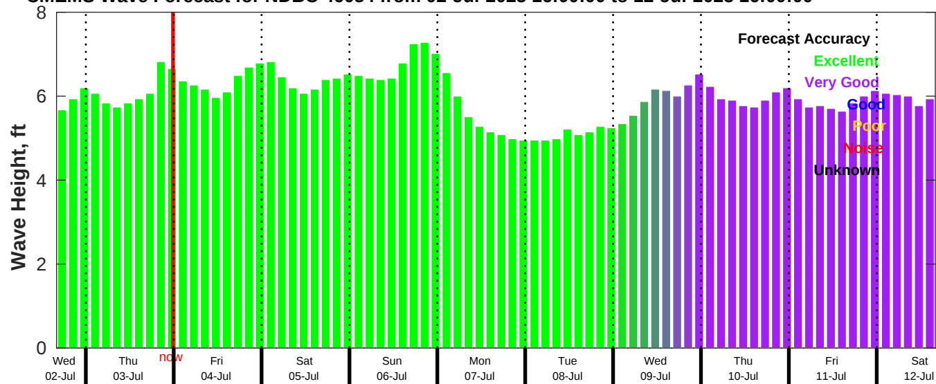
CMEMS Wave Forecast for NDBC 46054 from 02-Jul-2025 16:00:00 to 12-Jul-2025 16:00:00
