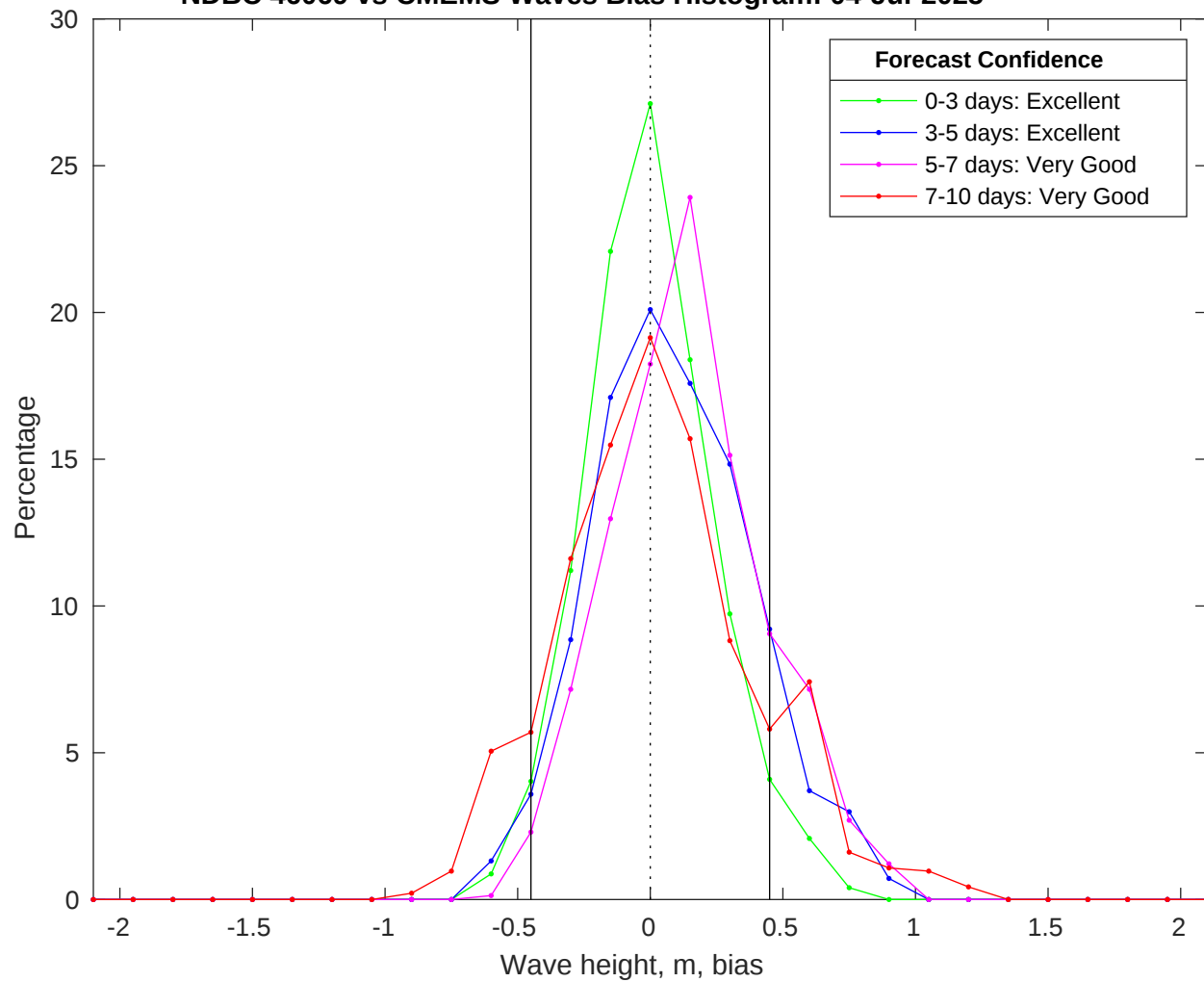
NDBC 46069 vs CMEMS Waves Bias Histogram: 04-Jul-2025
