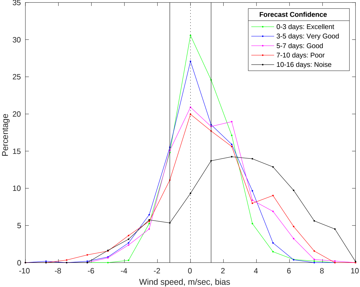
NDBC 46069 vs GFS Winds Bias Histogram: 04-Jul-2025
