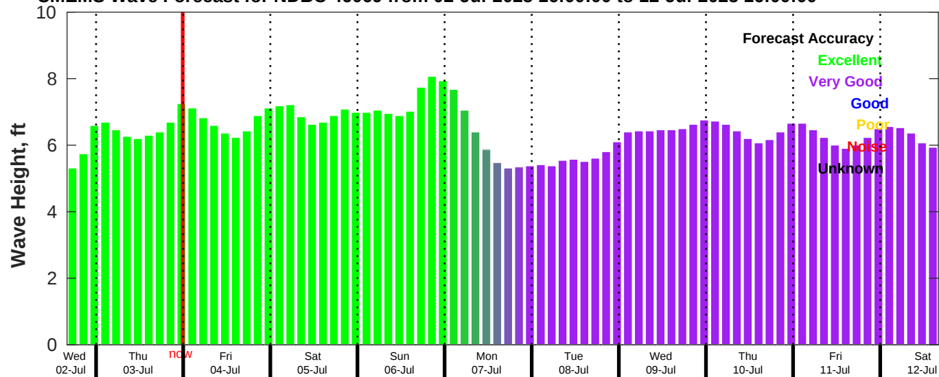
CMEMS Wave Forecast for NDBC 46069 from 02-Jul-2025 16:00:00 to 12-Jul-2025 16:00:00
