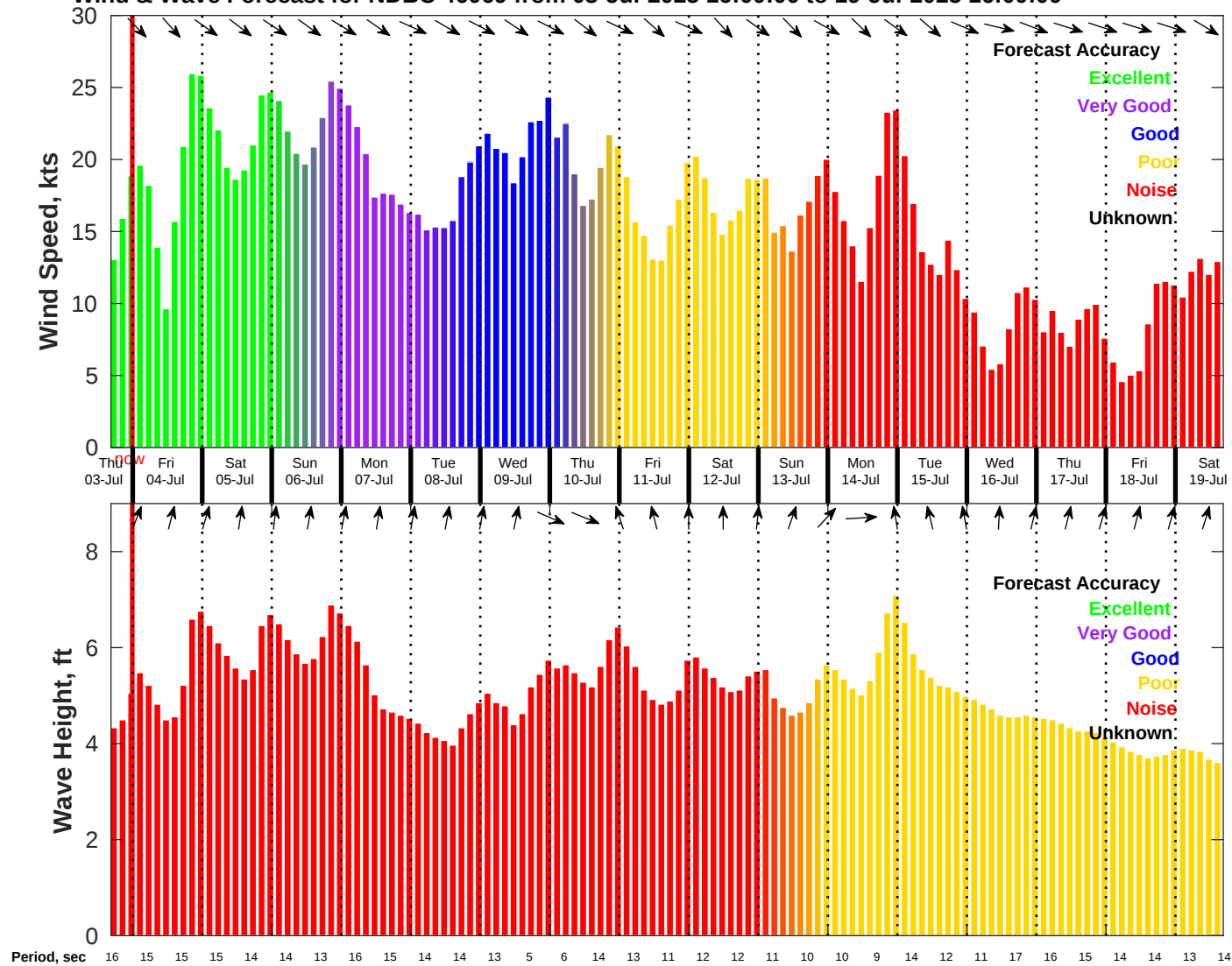
Wind & Wave Forecast for NDBC 46069 from 03-Jul-2025 16:00:00 to 19-Jul-2025 16:00:00
