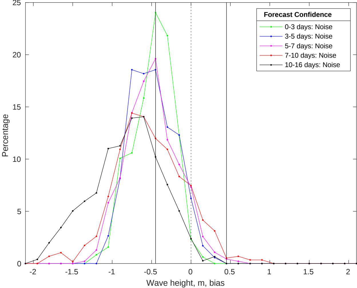
NDBC 51209 vs GFS Waves Bias Histogram: 04-Jul-2025
