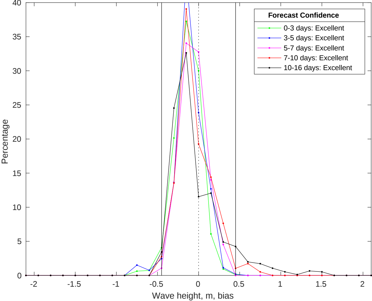
NDBC 52212 vs GFS Waves Bias Histogram: 04-Jul-2025
