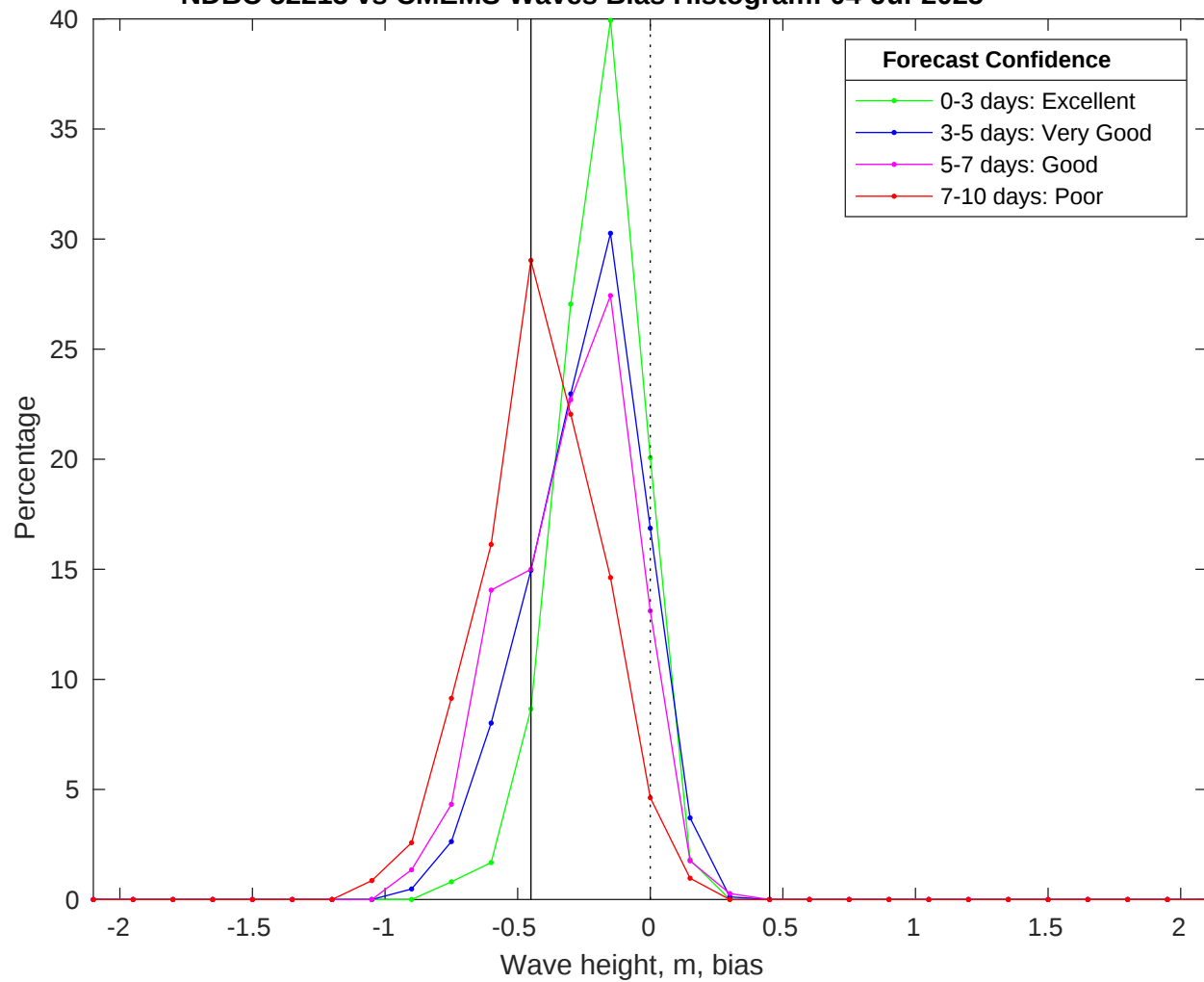
NDBC 52213 vs CMEMS Waves Bias Histogram: 04-Jul-2025
