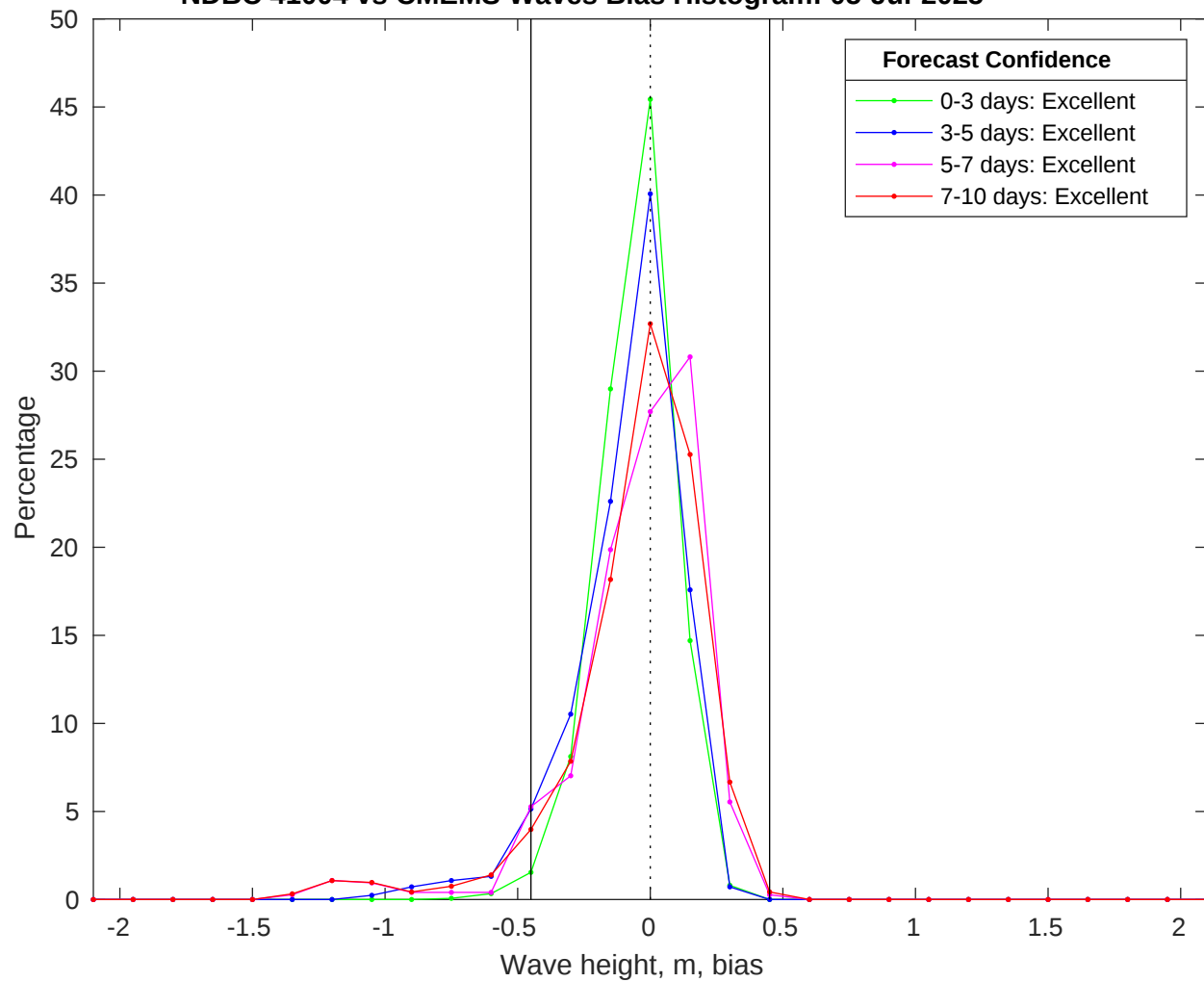
NDBC 41004 vs CMEMS Waves Bias Histogram: 05-Jul-2025
