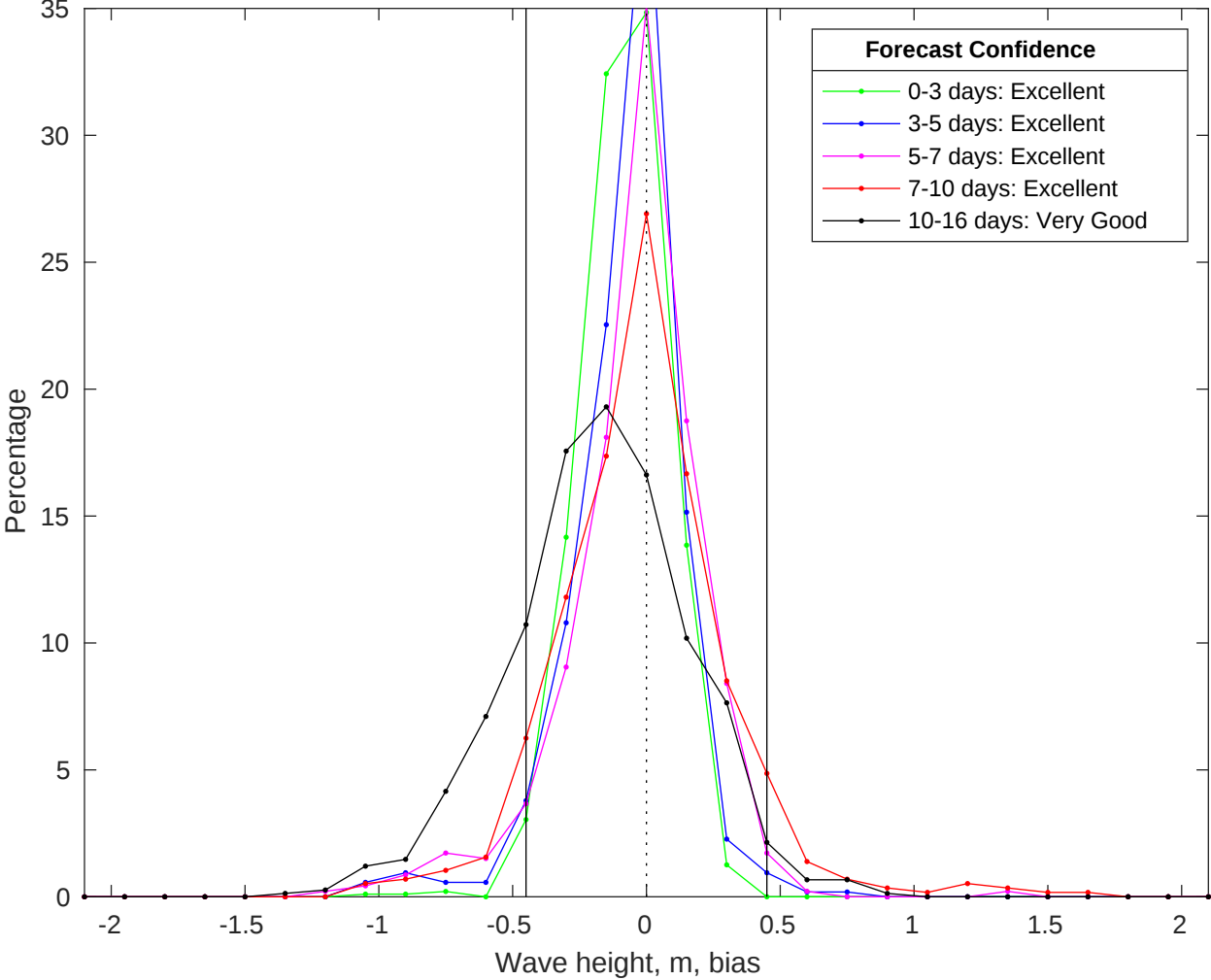
NDBC 41004 vs GFS Waves Bias Histogram: 05-Jul-2025
