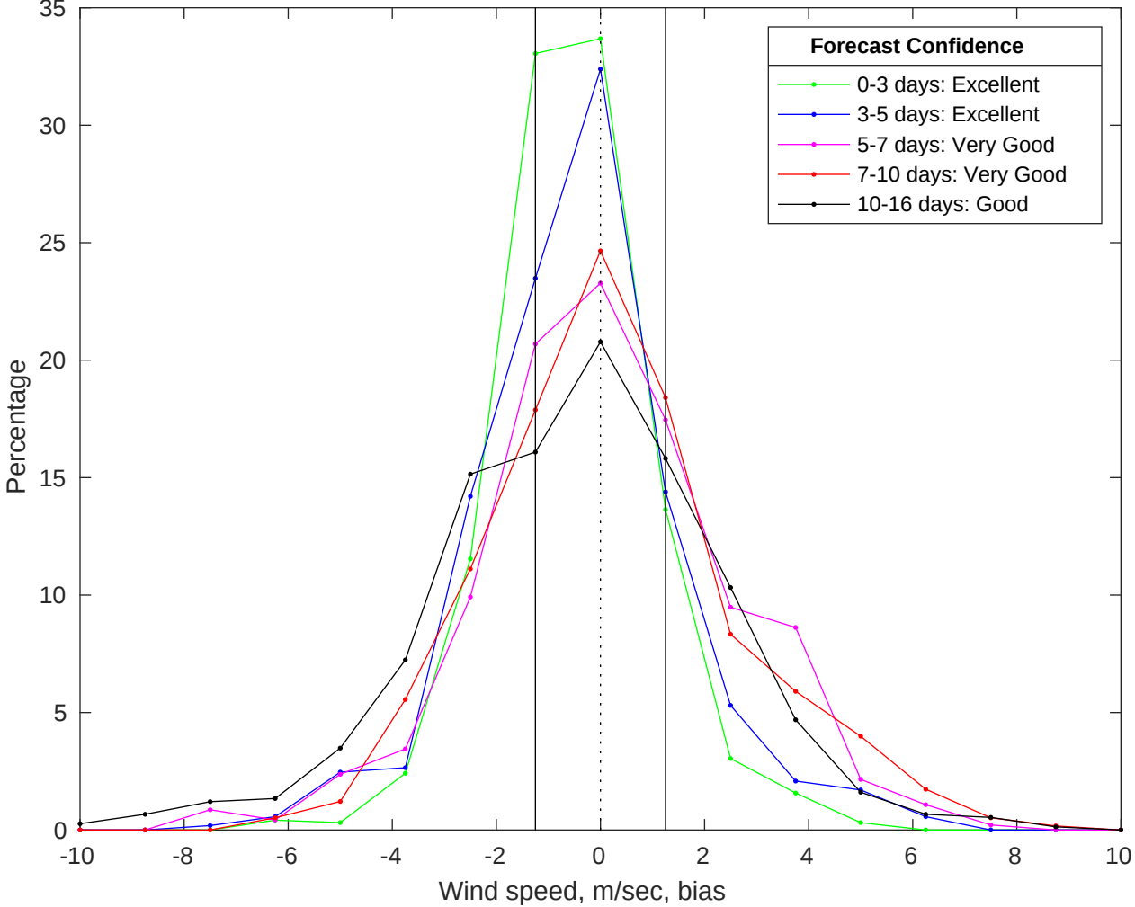
NDBC 41004 vs GFS Winds Bias Histogram: 05-Jul-2025
