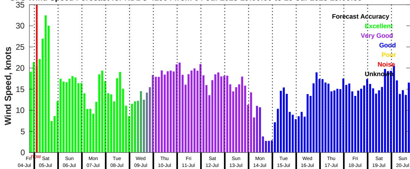
GFS Wind Speed Forecast for NDBC 41004 from 04-Jul-2025 19:00:00 to 20-Jul-2025 19:00:00
