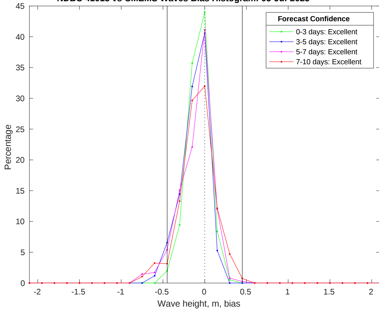
NDBC 41013 vs CMEMS Waves Bias Histogram: 05-Jul-2025
