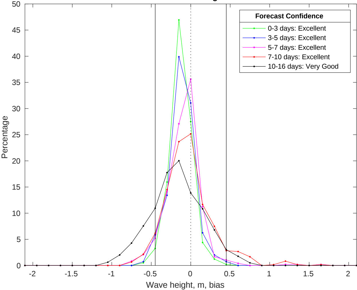
NDBC 41013 vs GFS Waves Bias Histogram: 05-Jul-2025
