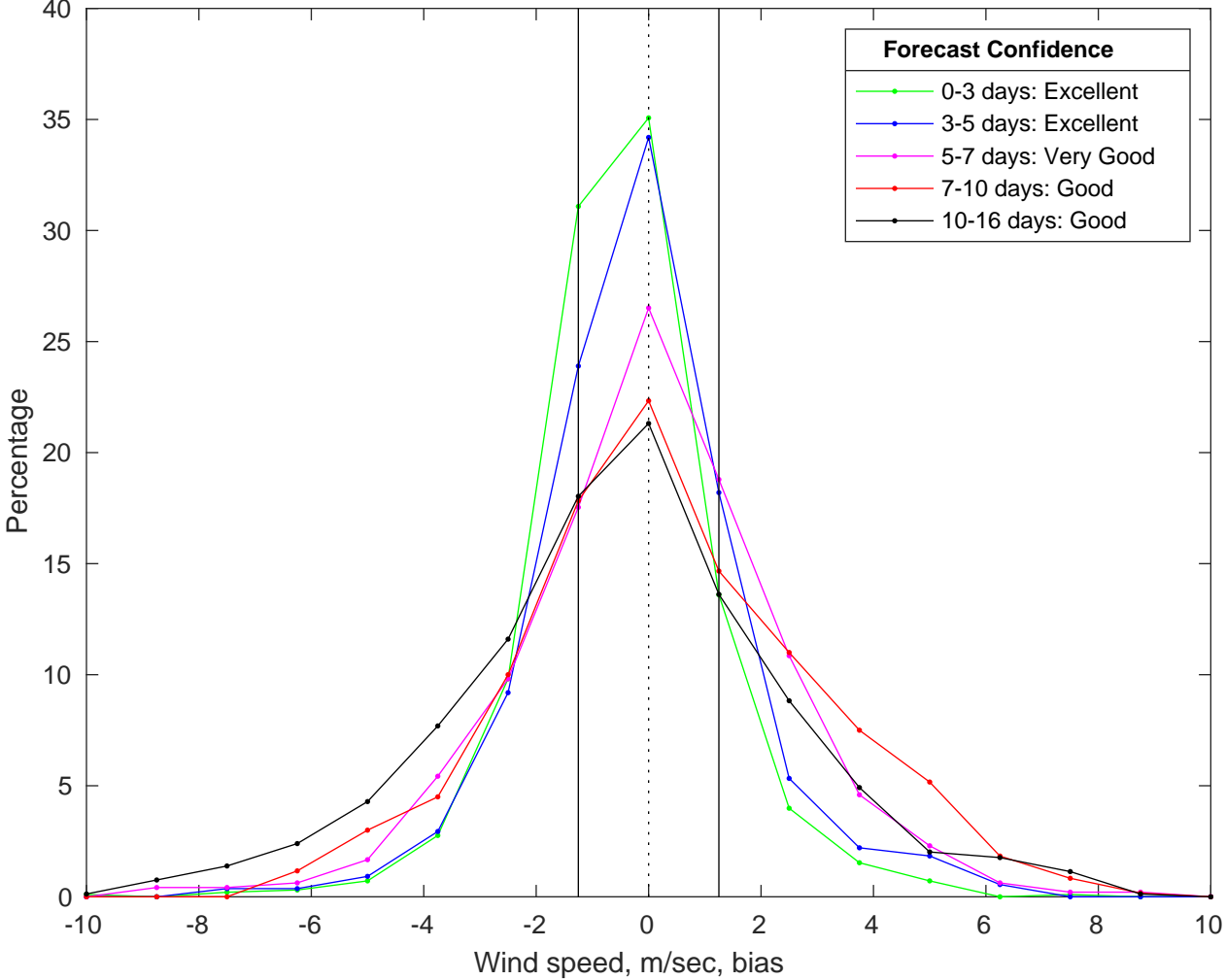
NDBC 41013 vs GFS Winds Bias Histogram: 05-Jul-2025
