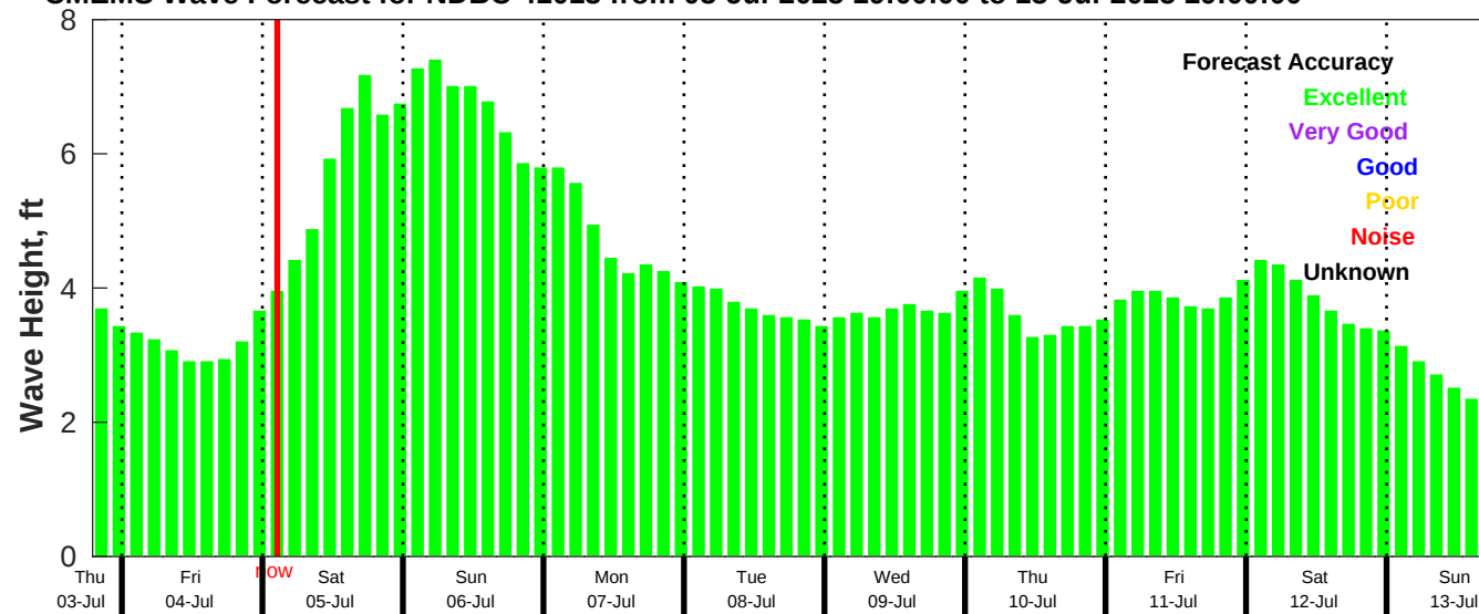
CMEMS Wave Forecast for NDBC 41013 from 03-Jul-2025 19:00:00 to 13-Jul-2025 19:00:00
