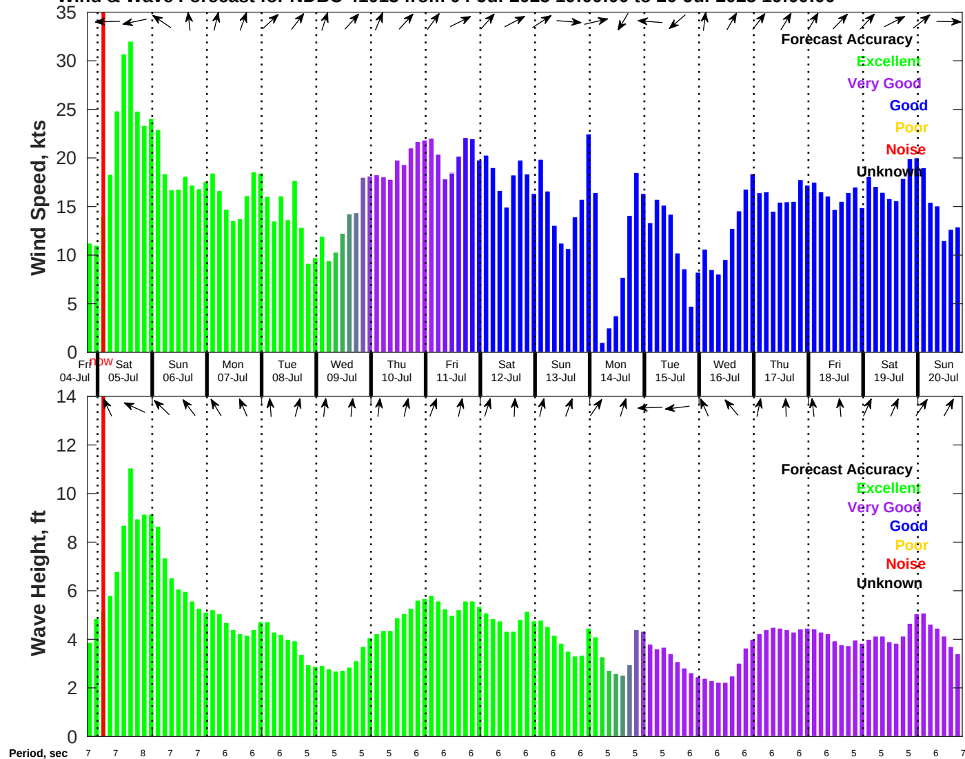
Wind & Wave Forecast for NDBC 41013 from 04-Jul-2025 19:00:00 to 20-Jul-2025 19:00:00
