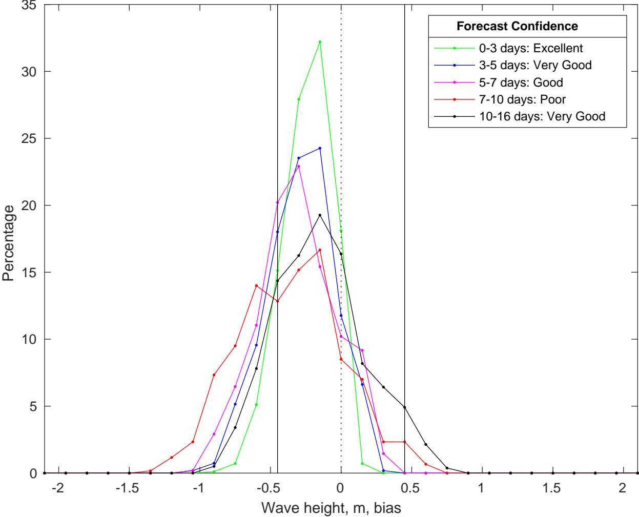
NDBC 41040 vs GFS Waves Bias Histogram: 05-Jul-2025
