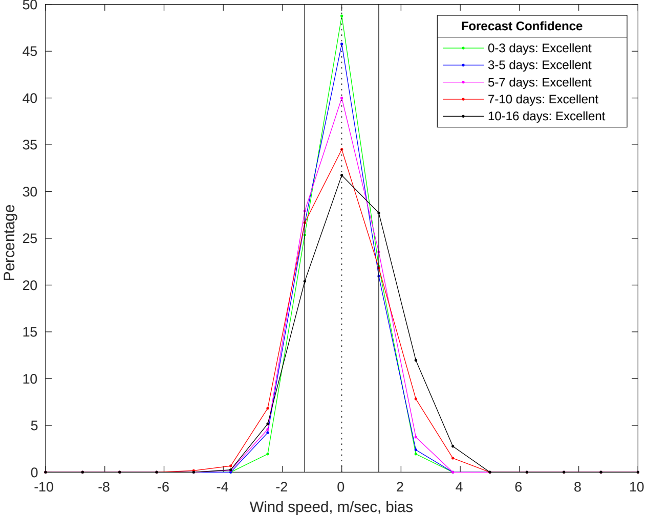
NDBC 41040 vs GFS Winds Bias Histogram: 05-Jul-2025
