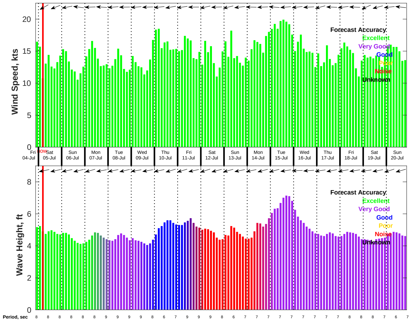
Wind & Wave Forecast for NDBC 41040 from 04-Jul-2025 21:00:00 to 20-Jul-2025 21:00:00
