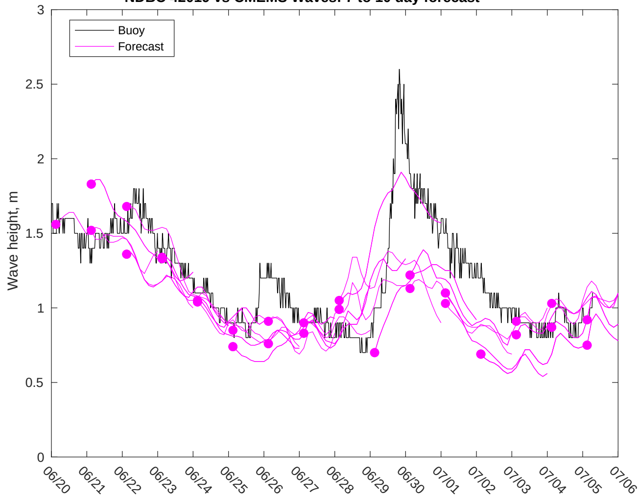
NDBC 42019 vs CMEMS Waves: 7 to 10 day forecast
