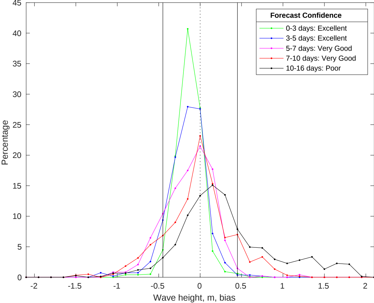
NDBC 42019 vs GFS Waves Bias Histogram: 05-Jul-2025
