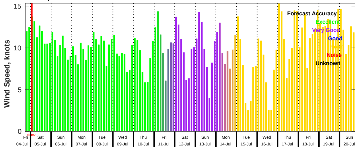
GFS Wind Speed Forecast for NDBC 42019 from 04-Jul-2025 18:00:00 to 20-Jul-2025 18:00:00
