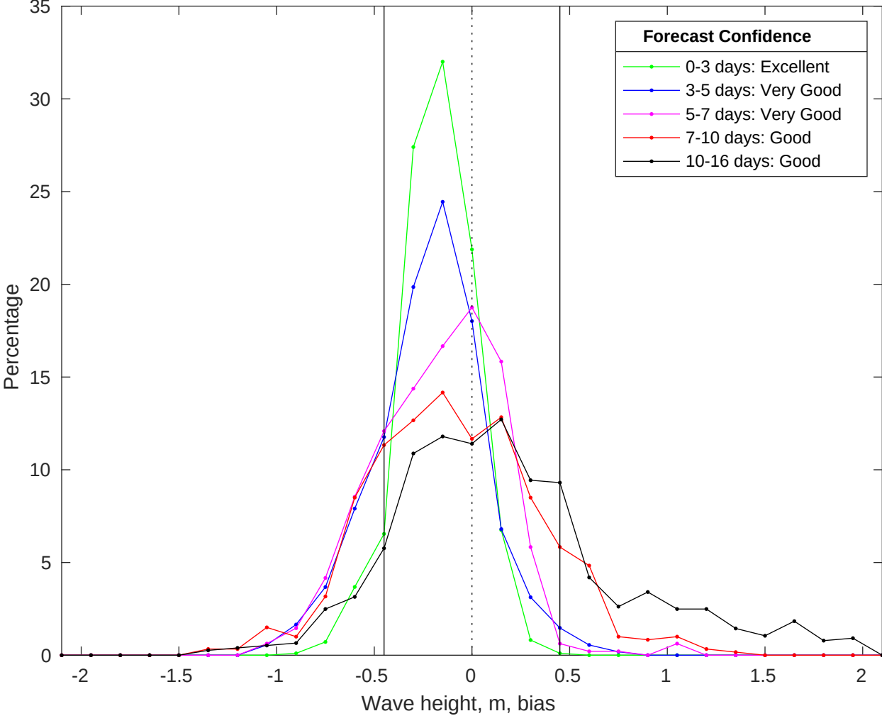
NDBC 42020 vs GFS Waves Bias Histogram: 05-Jul-2025
