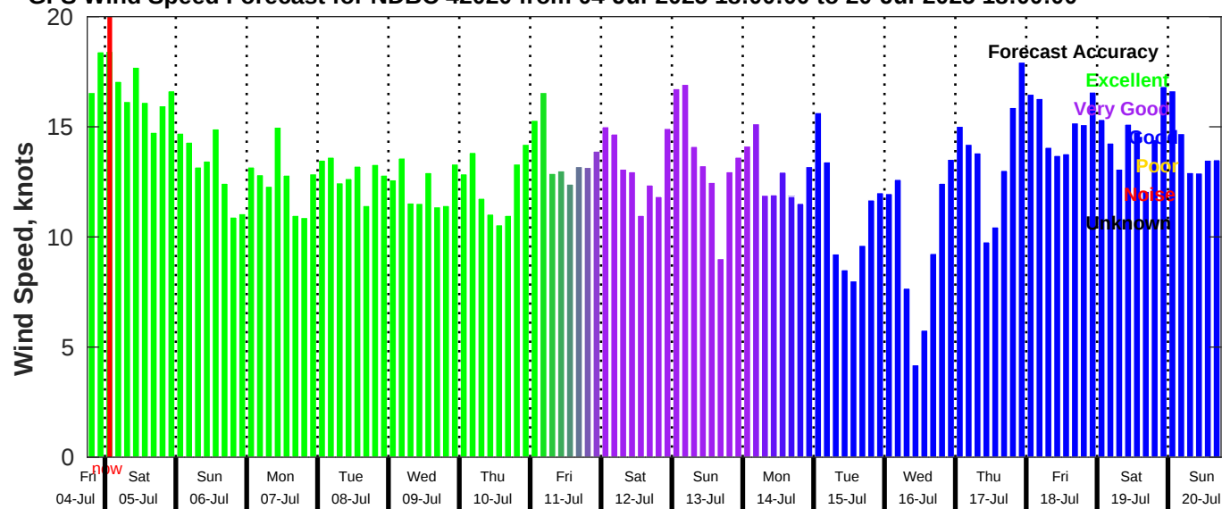
GFS Wind Speed Forecast for NDBC 42020 from 04-Jul-2025 18:00:00 to 20-Jul-2025 18:00:00
