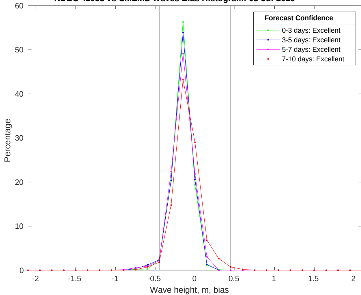
NDBC 42035 vs CMEMS Waves Bias Histogram: 05-Jul-2025
