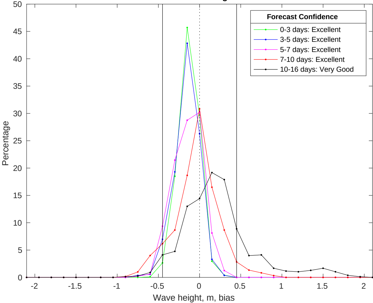
NDBC 42035 vs GFS Waves Bias Histogram: 05-Jul-2025
