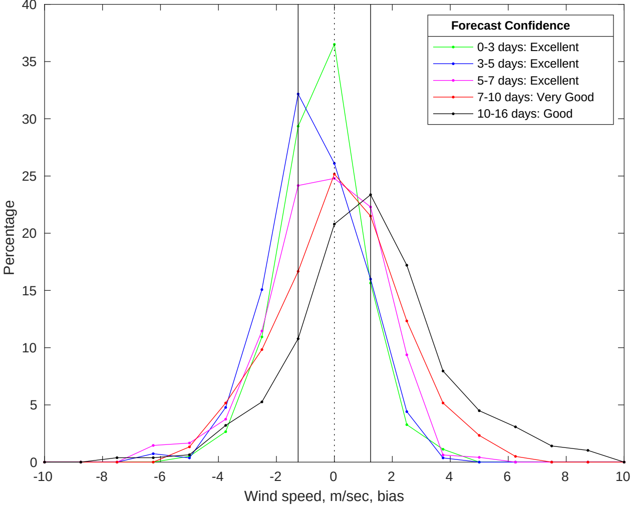
NDBC 42035 vs GFS Winds Bias Histogram: 05-Jul-2025
