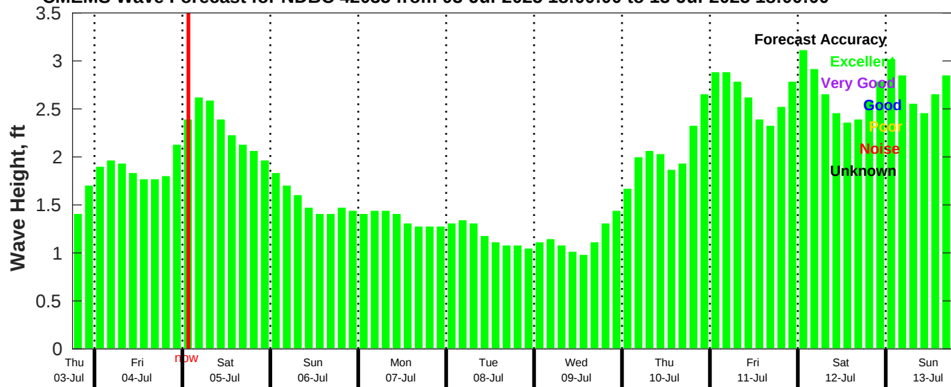
CMEMS Wave Forecast for NDBC 42035 from 03-Jul-2025 18:00:00 to 13-Jul-2025 18:00:00
