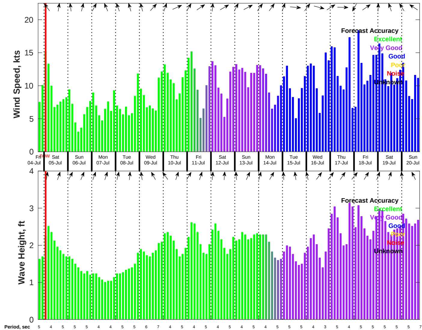
Wind & Wave Forecast for NDBC 42035 from 04-Jul-2025 18:00:00 to 20-Jul-2025 18:00:00
