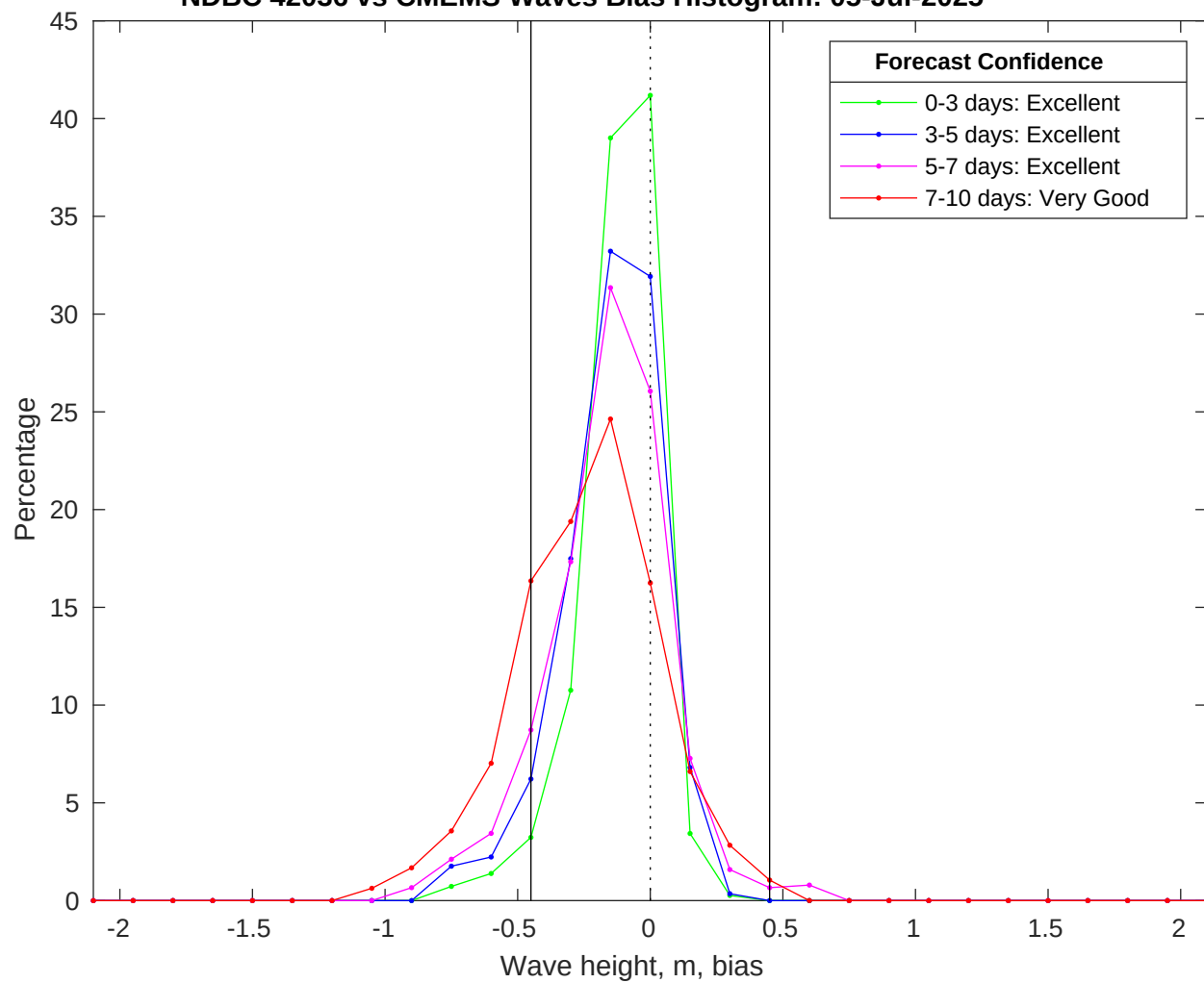
NDBC 42036 vs CMEMS Waves Bias Histogram: 05-Jul-2025
