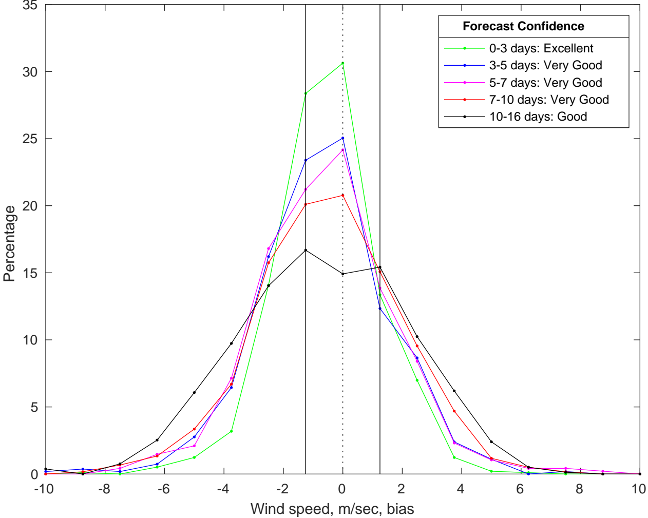
NDBC 42036 vs GFS Winds Bias Histogram: 05-Jul-2025
