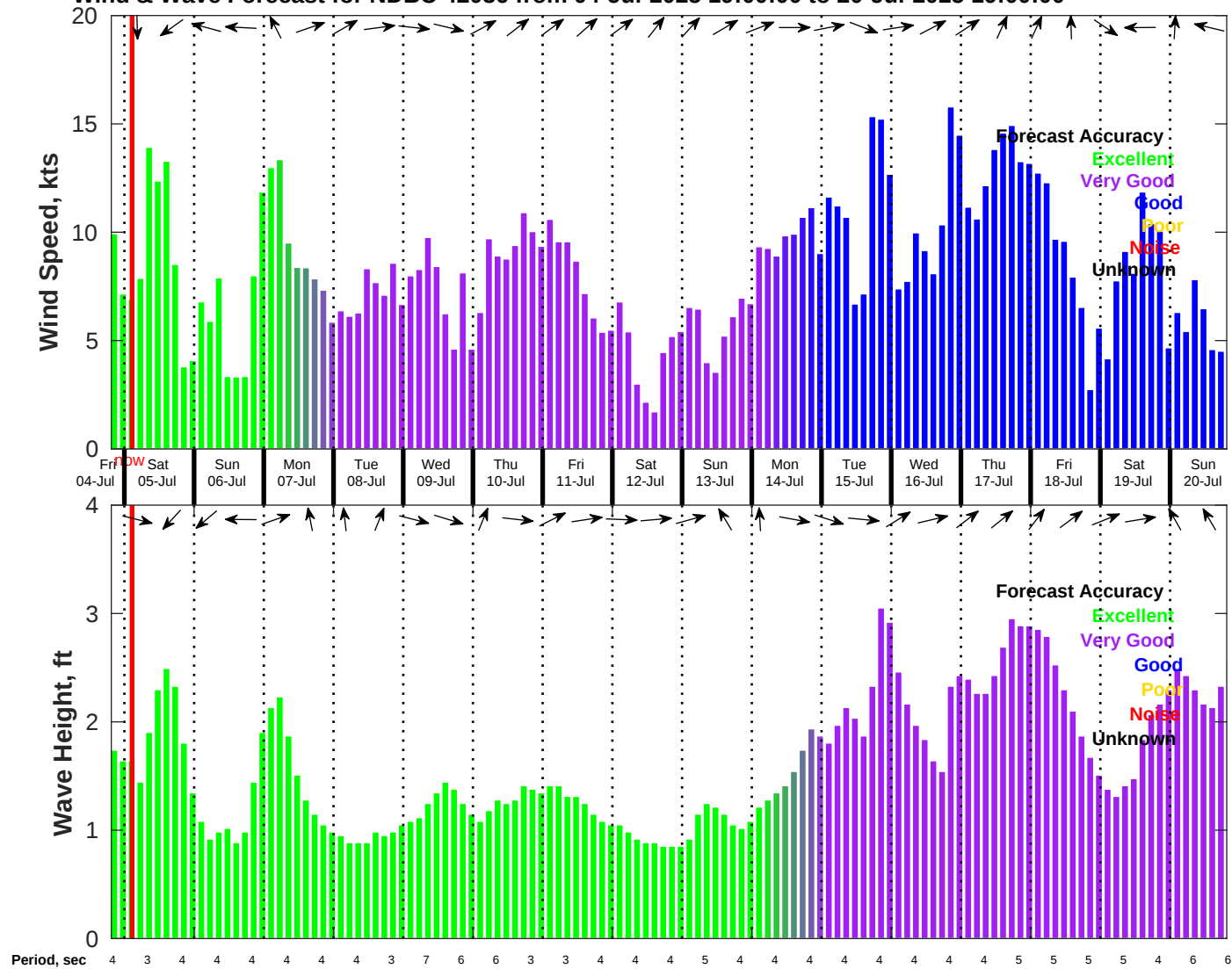
Wind & Wave Forecast for NDBC 42036 from 04-Jul-2025 19:00:00 to 20-Jul-2025 19:00:00
